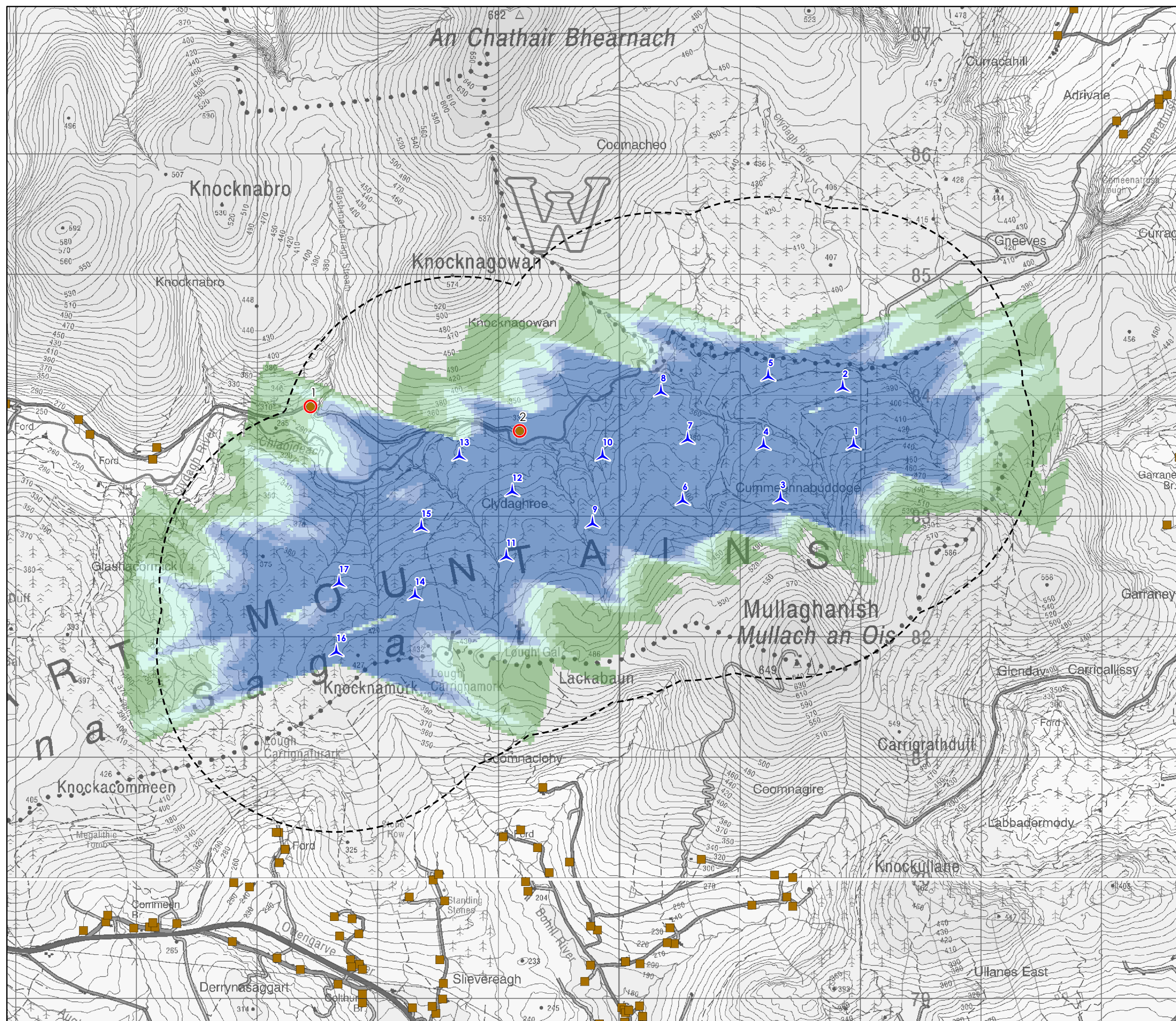
Figure 15-1b Shadow Flicker Assessment - Minimum Rotor Diameter
